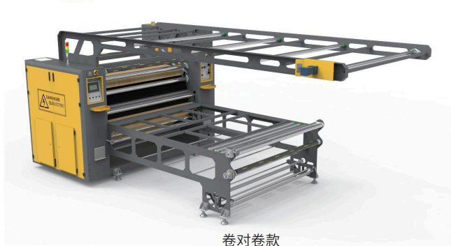
卷对卷款 Roll-to-roll standard machine
